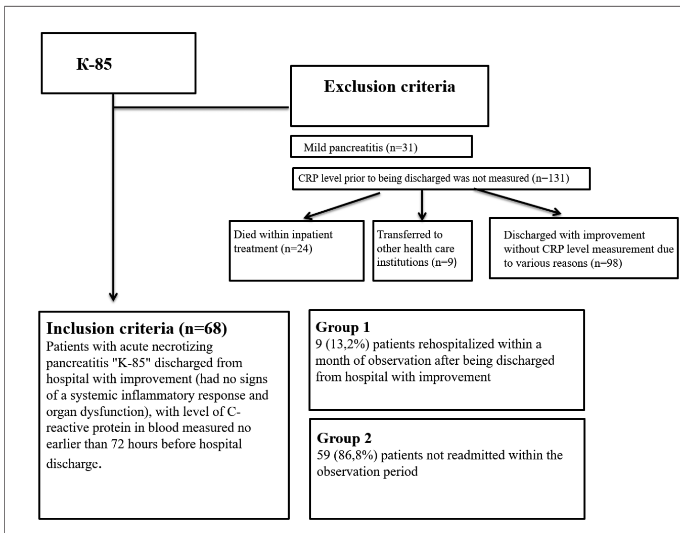
Fig. 1. Study Design
