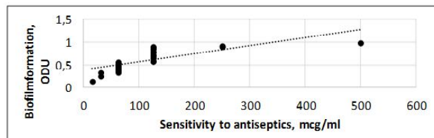
Fig. 4. Correlation between biofilm formation and sensitivity to chlorhexidine of clinical strains of P.aeruginosa (n=30).
