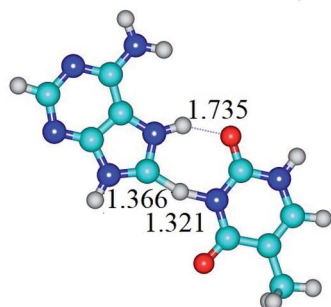
TS A·T*O 2 (rwH) to A*C 8 ·T(rwH) ( \nu_i = 1129.2 \text{ i cm}^{-1} )
