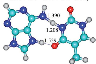
TS A·T*(rwH) to A*N 7 ·T(rwH) ( \nu_i = 727.4 \text{ i cm}^{-1} )
